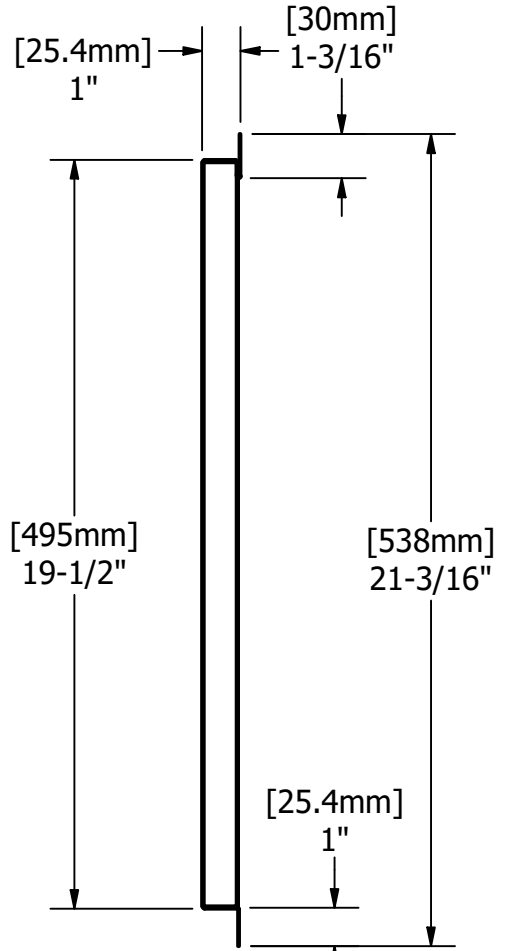
SECTION B-B DETAIL 1:5
