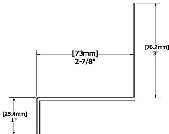
No. M54H.B (BB & RBB) Double drip flashing w/90 degrees angle
