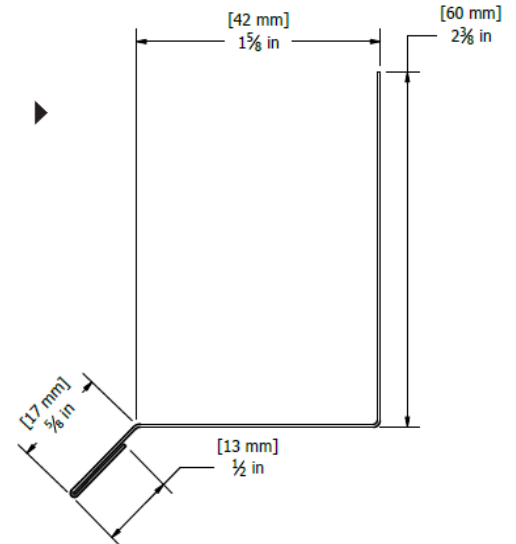
No. M53J (SPC1.2, SPC1.3) Double drip
