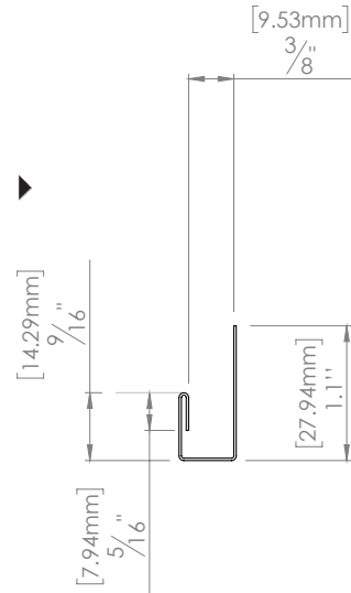
No. M01C ((HWP, HW, HWB & MS 14) J Trim
