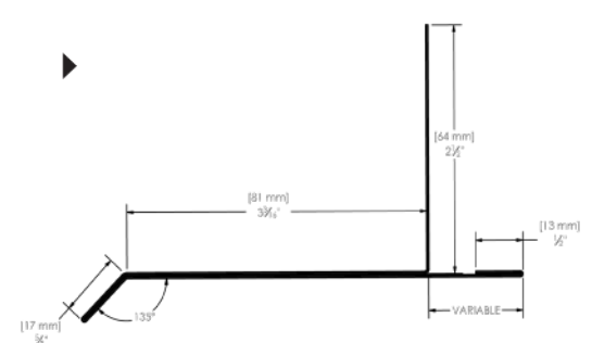
No. M56J (SPC1.2, SPC1.3) Extended drip flashing w/variable
