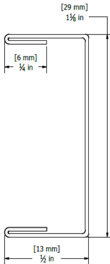
No. M06I (SPC1.1) Batten trim filler
