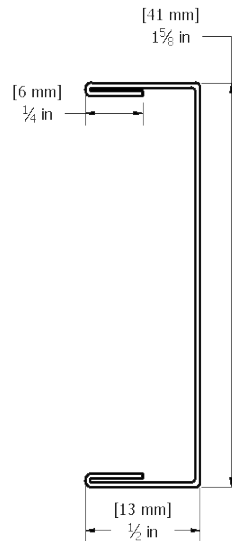
No. M06J (SPC1.2, SPC1.3) Batten trim filler
