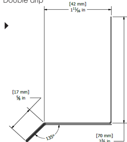
No. M53J (SPC1.2, SPC1.3) Double drip
