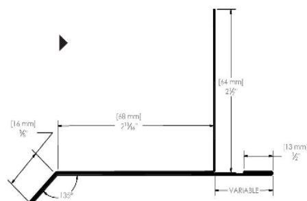
No. M56I (SPC1.1) Extended drip flashing w/variable
