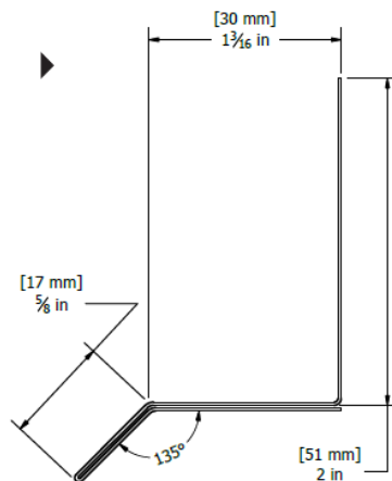
No. M53I (SPC1.1) Double drip
