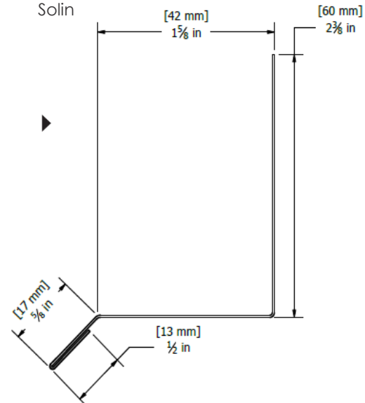
No. M53J (SPC1.2, SPC1.3) Solon double
