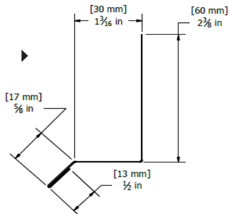
No. M50I (SPC1.1) Solon
