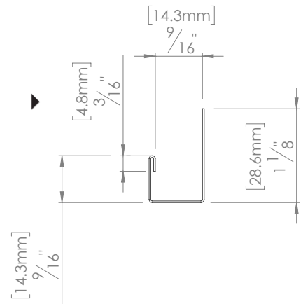
No. M01D (NW & NWM) J Trim
