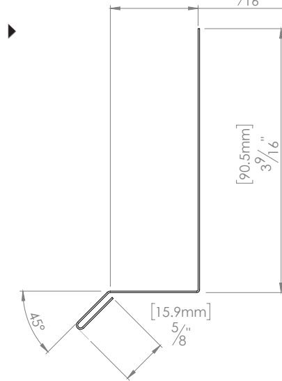
No. M50G (POL, VS, MB) [30.2mm] Solin
