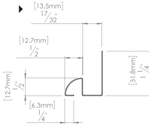
No. M53CD (HWP, HW, HWB, MS 14, NW & NWM) Solin double
