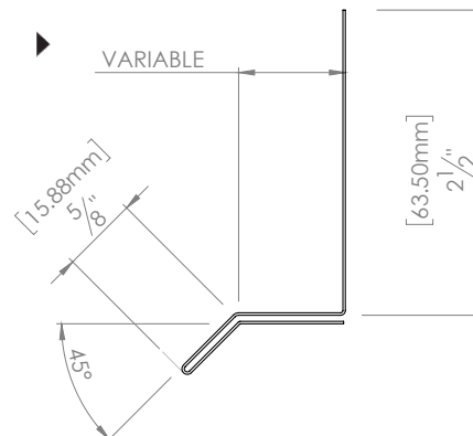
No. M55G (POL, VS, MB) Solin double variable
