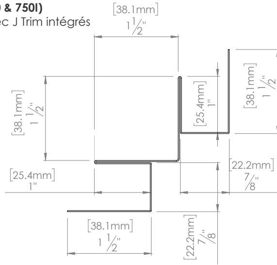
No. M53E (MS750 & 750I) Solain double
