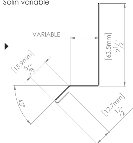
No. M52CD (HWP, HW, HWB, MS 14, NW & NWM) Solin variable
