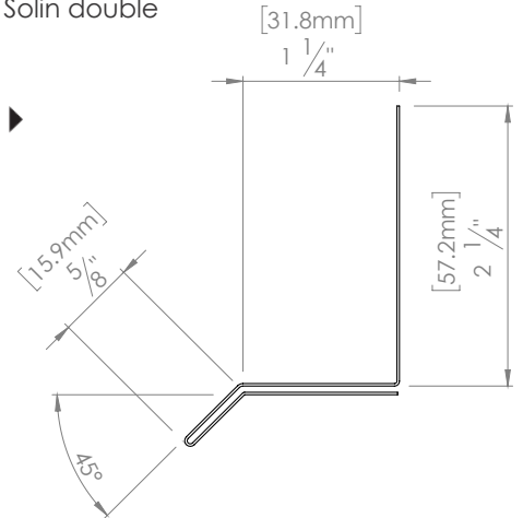
No. M53E (MS750 & 750I) Solain double
